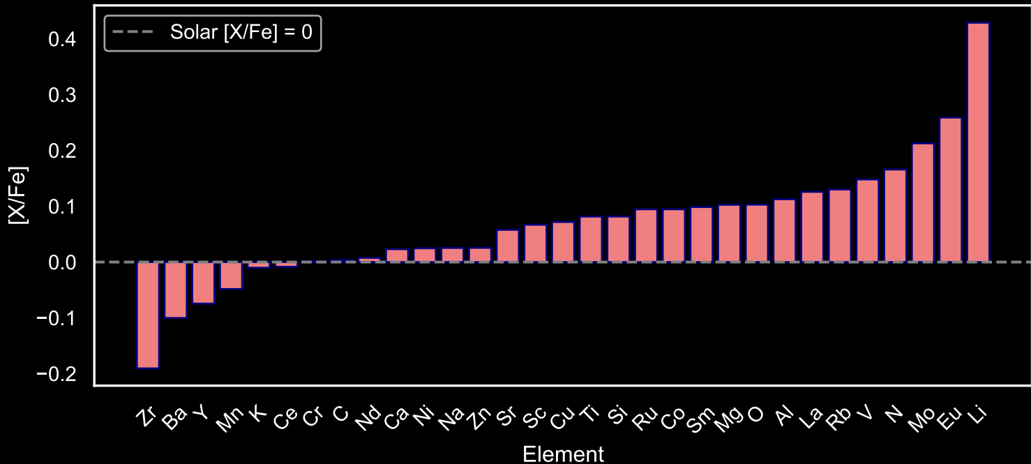
Abundance Pattern for GALAH Star Field [86] (N=210)
