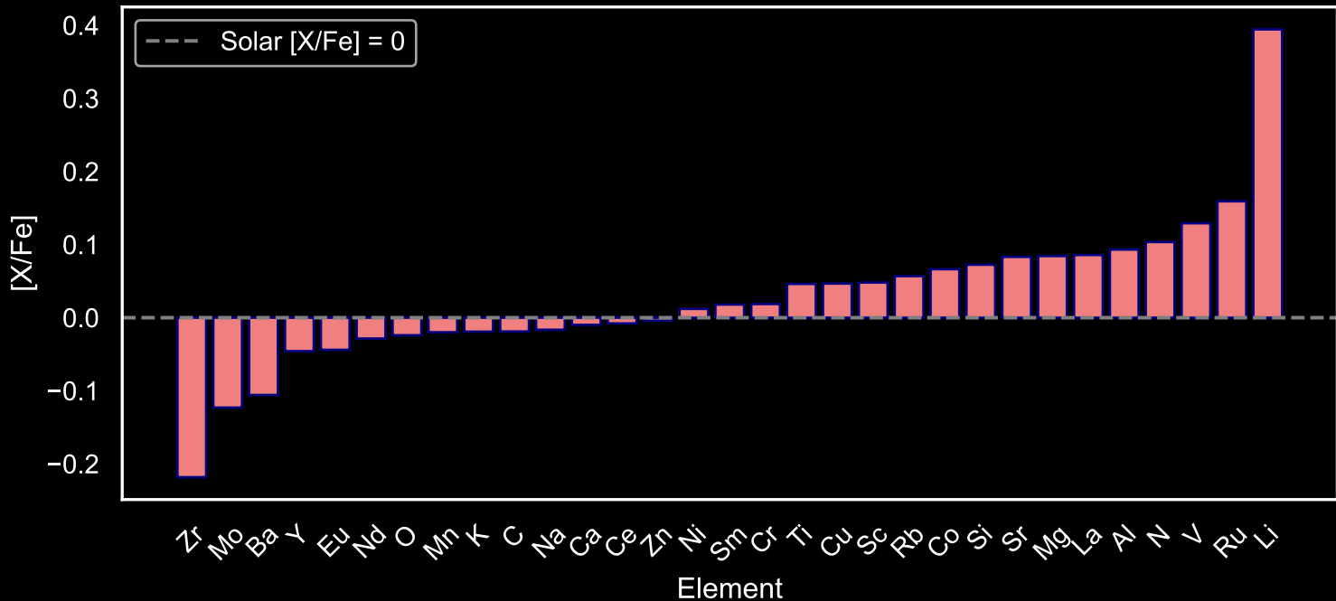
Abundance Pattern for GALAH Main Sequence Stars: Star Field [86] (N=103)
