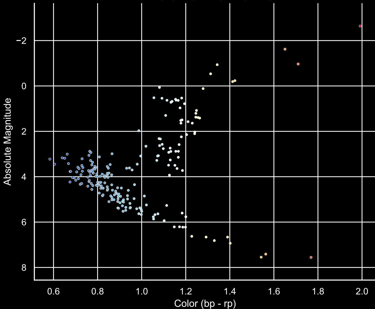
GALAH Hertzsprung-Russell Diagram Field [86] Ra [345.05] Dec [-70.98]
