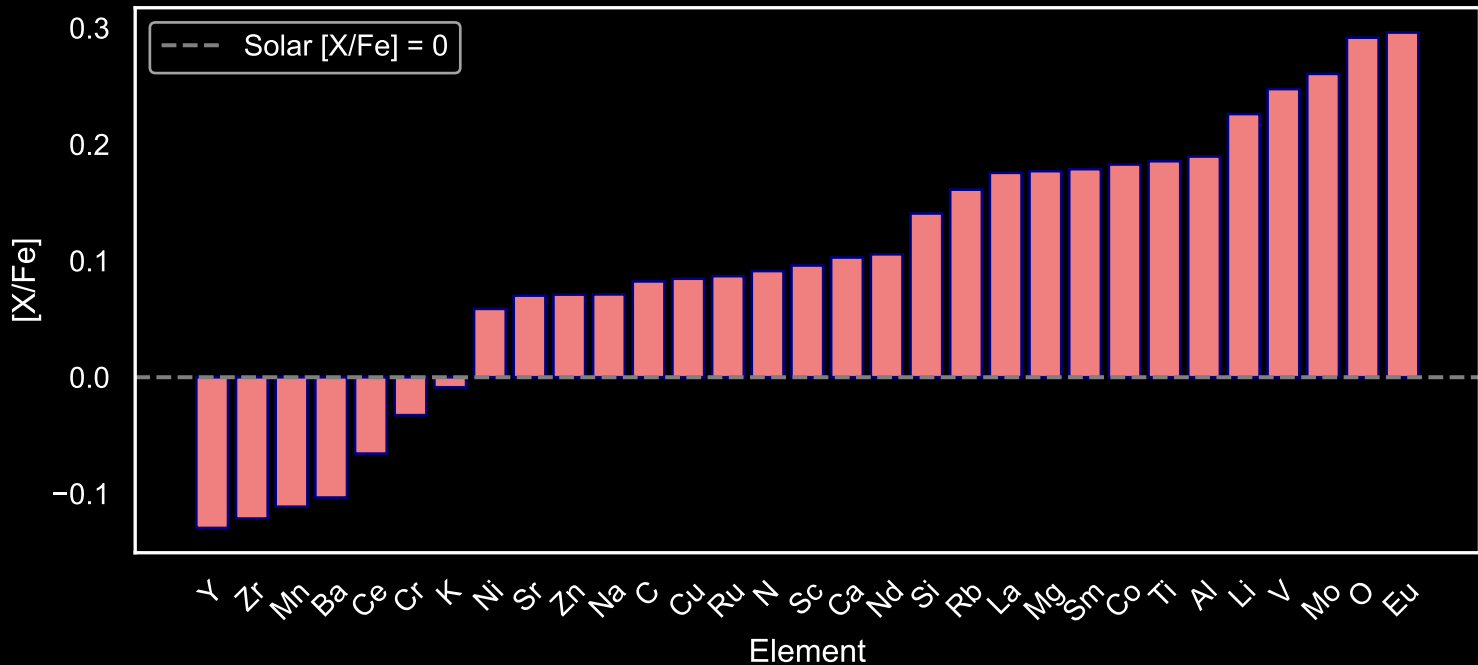
Abundance Pattern for GALAH Red Giants: Star Field [86] (N=54)
